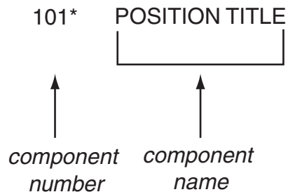
Figure 2.1 Schema Components
